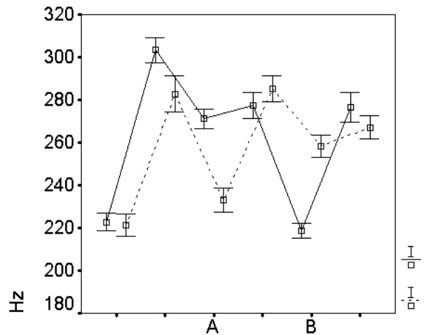
Figure 5: Means of L-H targets at left edge of Nouns 1-3 in SOV Structure I (full) and II (dotted) for KX
