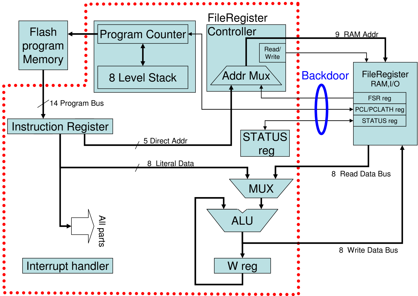
Fig.6 Block diagram(modified)
